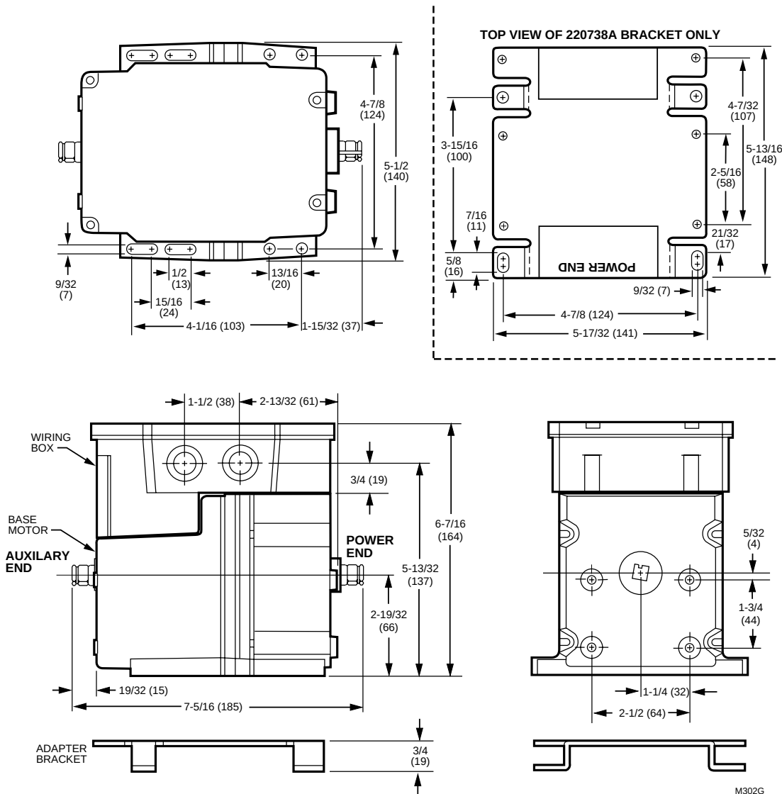
Fig. 1. M6284, M6294 mounting dimensions in in. (mm).
