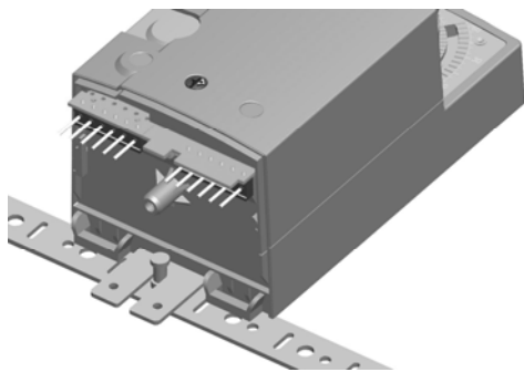
Fig. 13. Actuator with access cover removed
